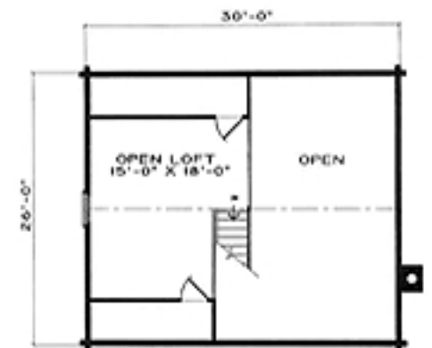
SUGGESTED 2ND FLOOR PLAN
